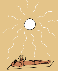
Ultraviolet light from the Sun 789THz–1.5PHz
